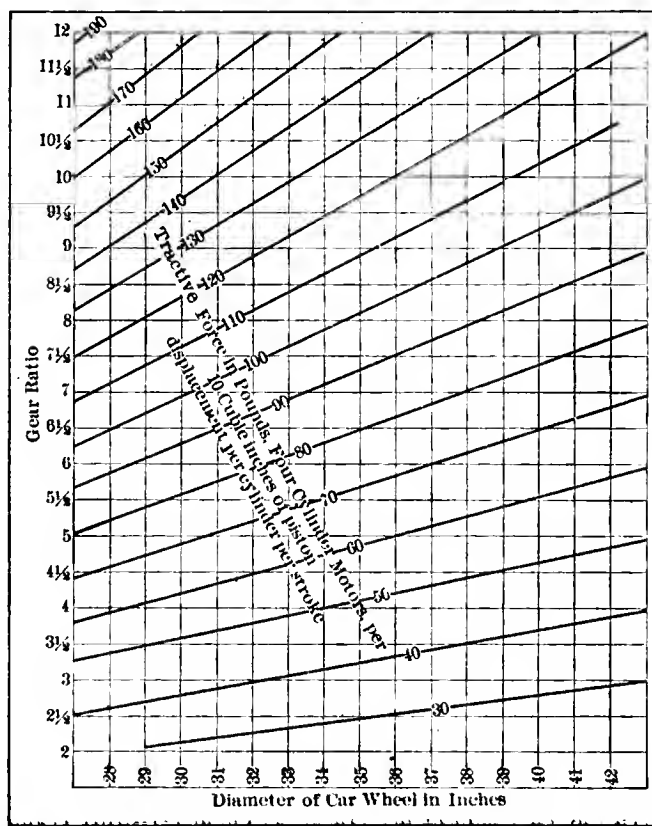
Fig. 1—Chart showing tractive force for various wheel diameters and gear ratios
